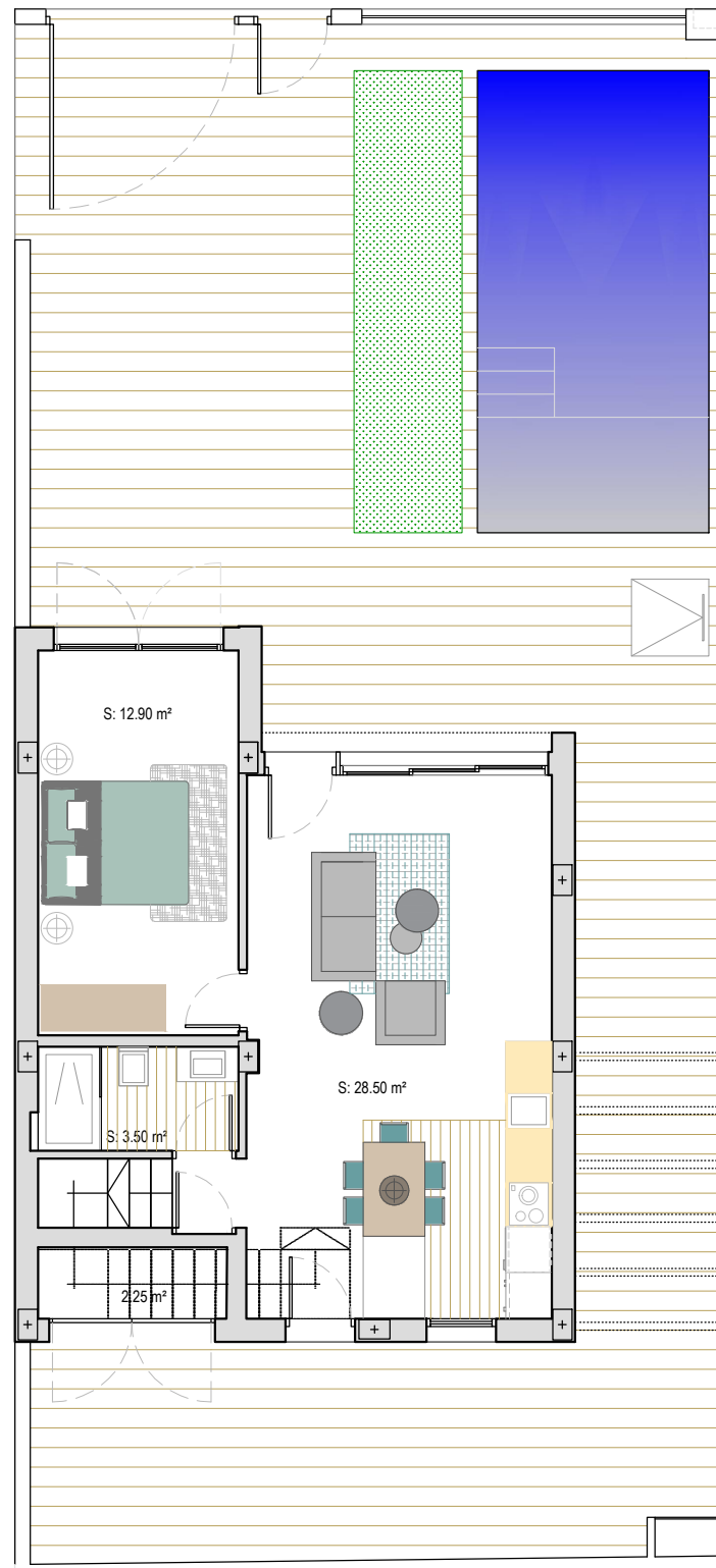
Ground floor
