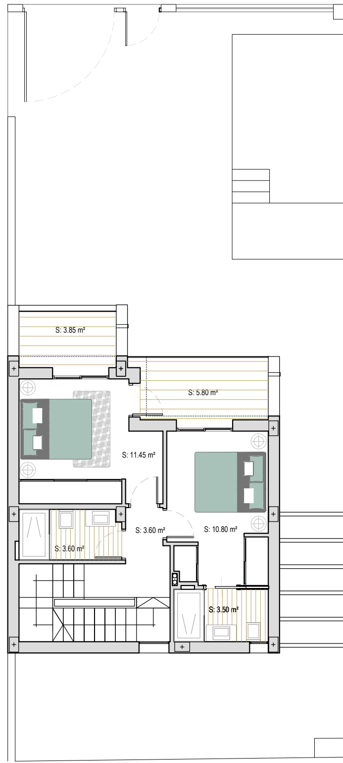
First floor
